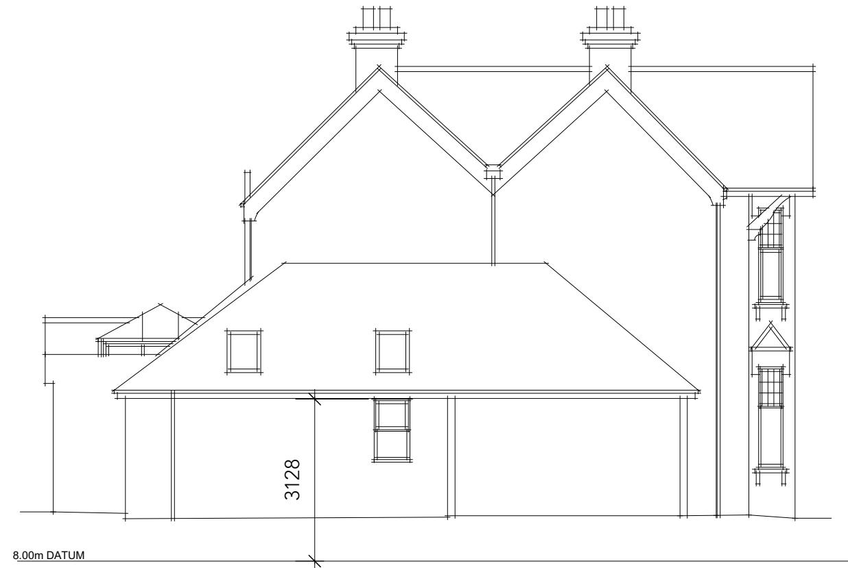
NORTH ELEVATION
