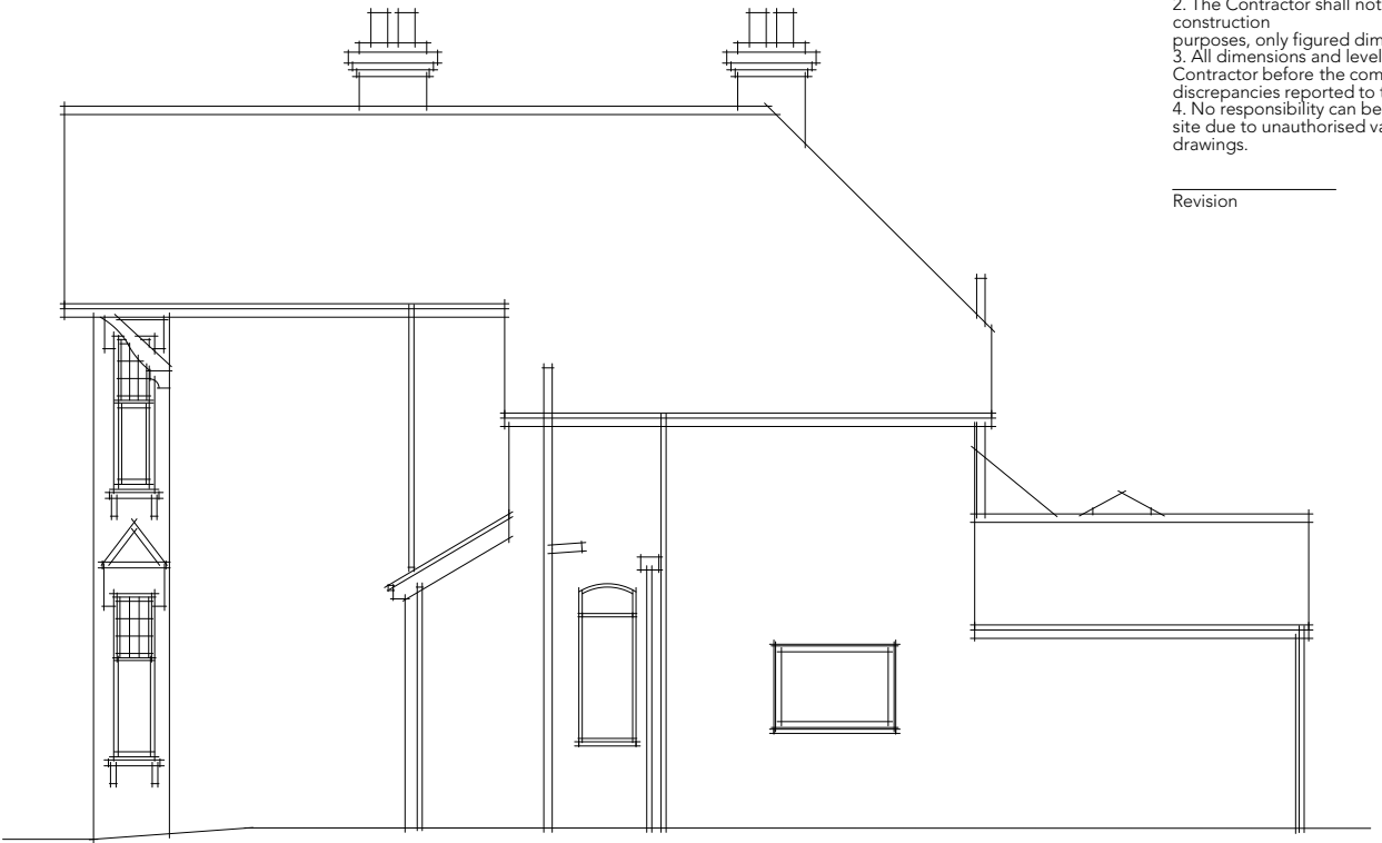
SOUTH ELEVATION
