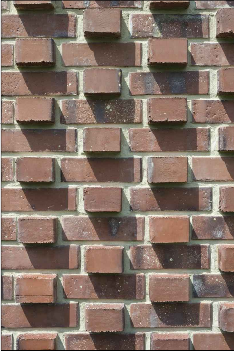
Flemish bond brick detailing
