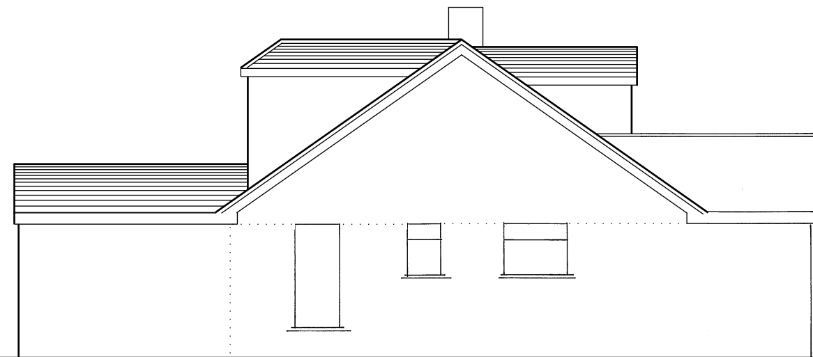
Proposed SE/Side Elevation
