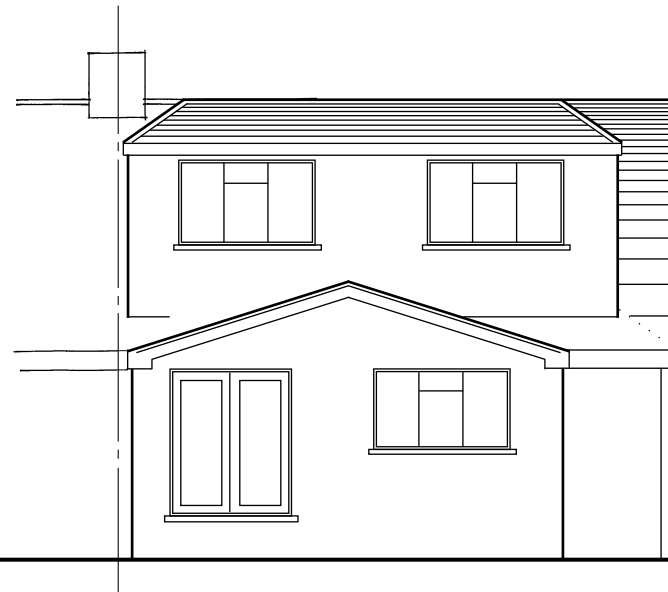
Proposed SW/Rear Elevation
