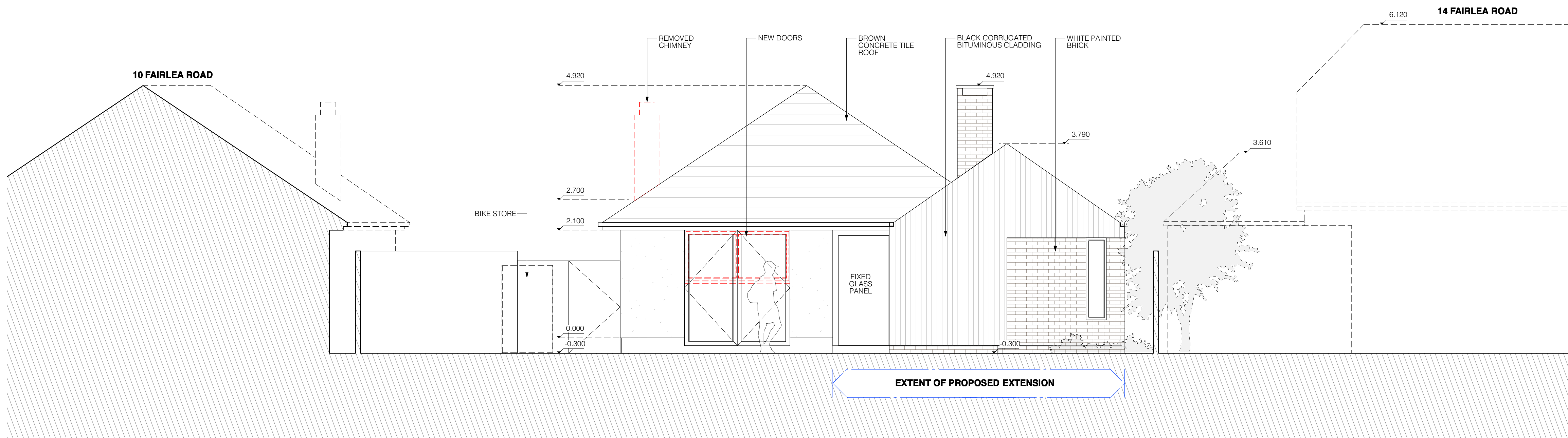
02 PROPOSED NORTHERN ELEVATION 1:50
