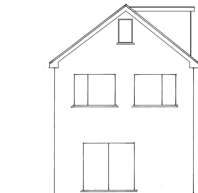
Proposed South/Rear Elevation
