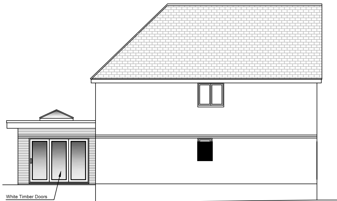
Rear Elevation
