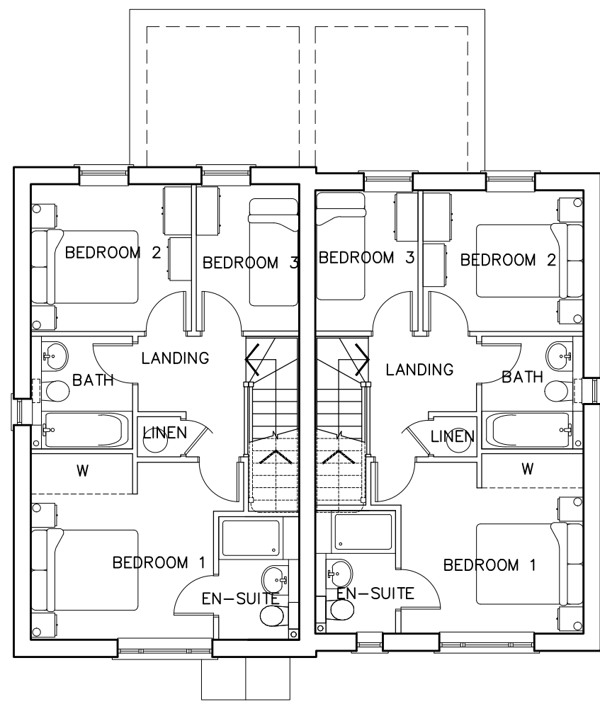
FIRST FLOOR
