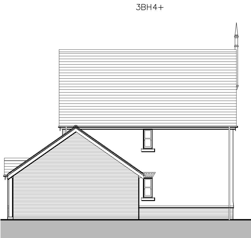
SIDE ELEVATION – D
