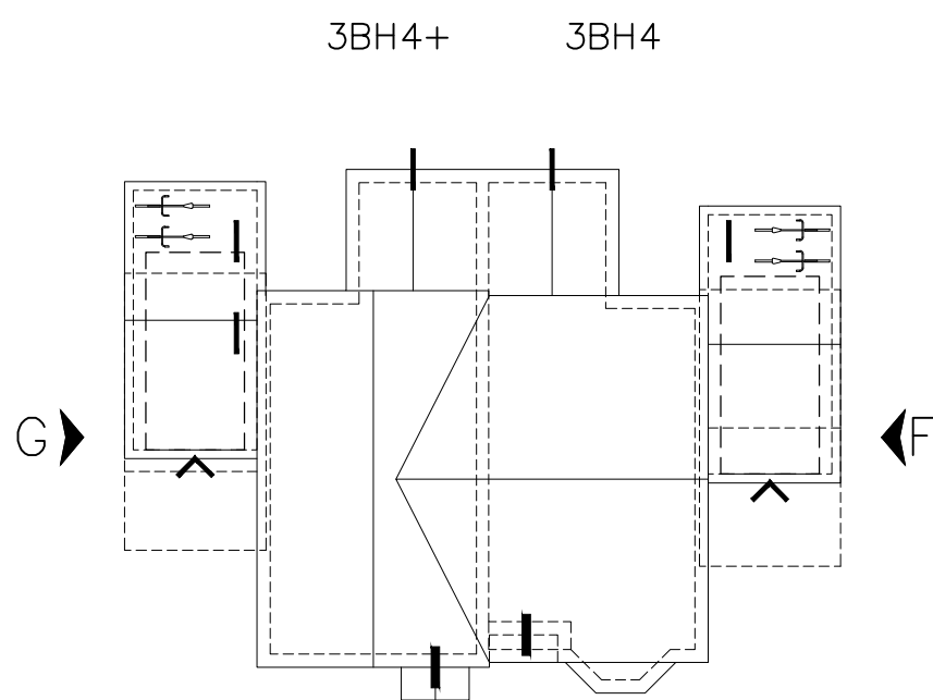
ROOF PLAN 1:200
