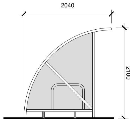
Side Elevation
