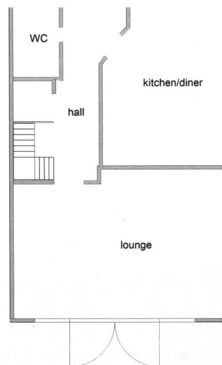
Existing Plan Elevation 1:100
