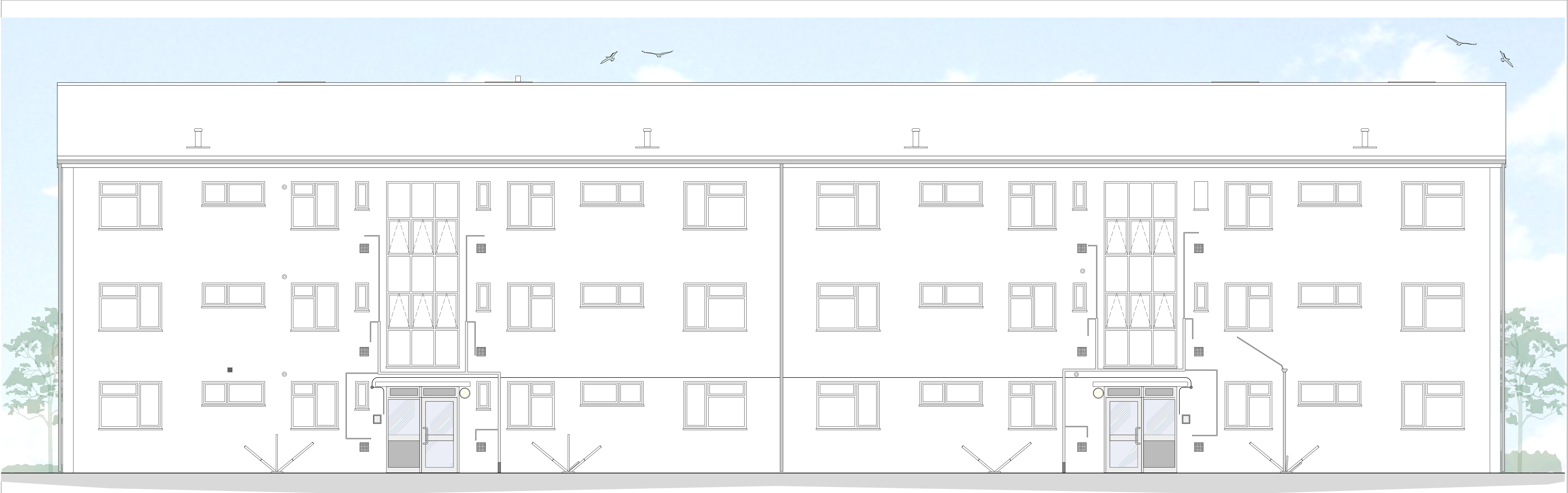
PROPOSED ELEVATION 2: FLATS 10-16 & FLATS 18-24A
