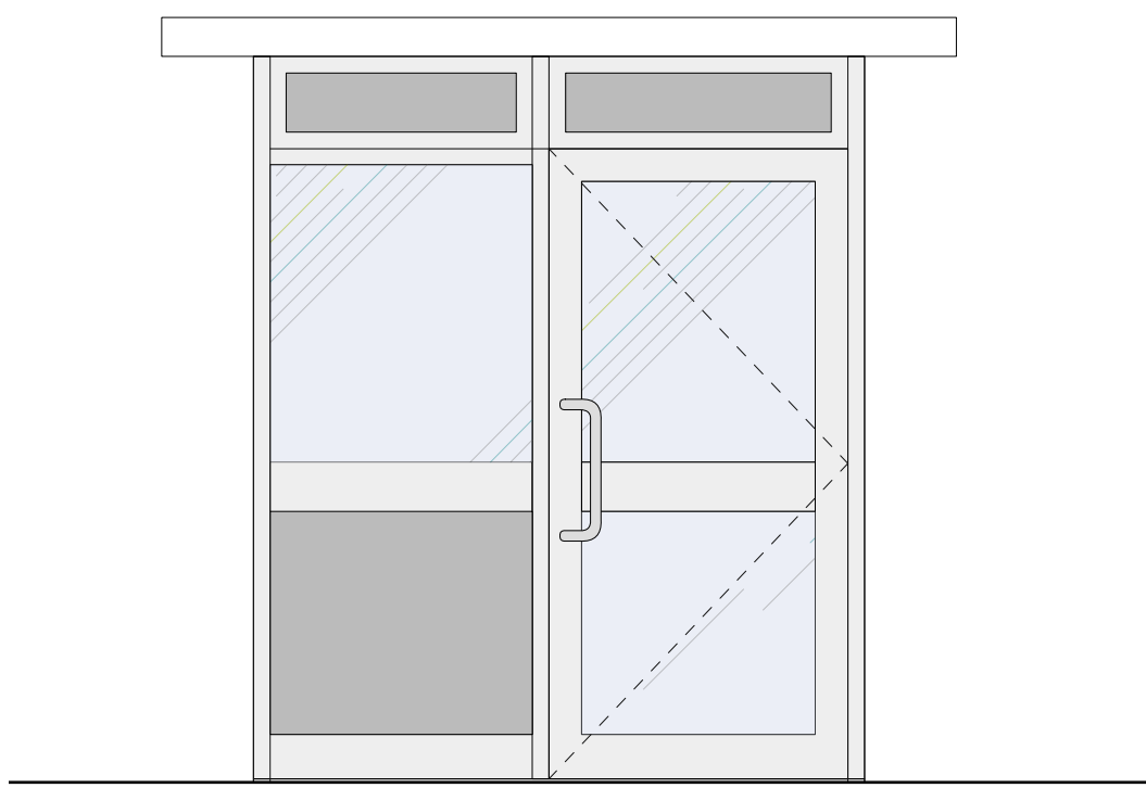
PROPOSED NEW ENTRANCE Scale 1:25 @ A1
