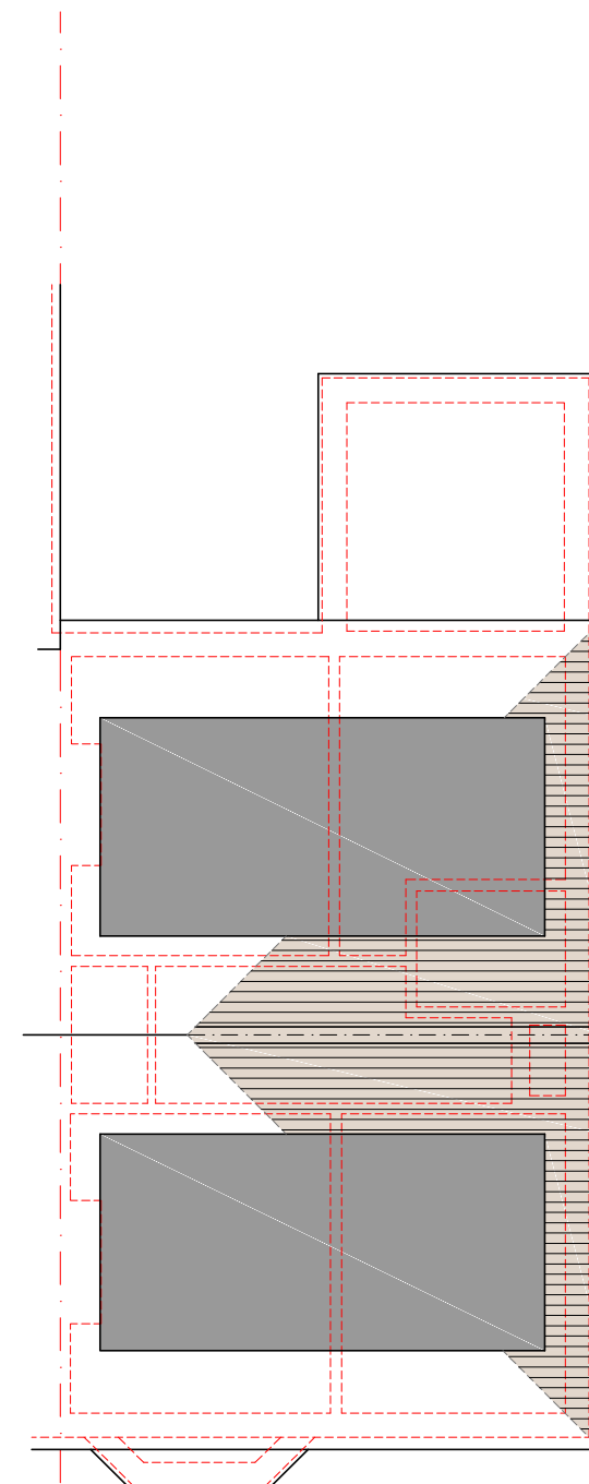
ROOF LAYOUT PLAN
