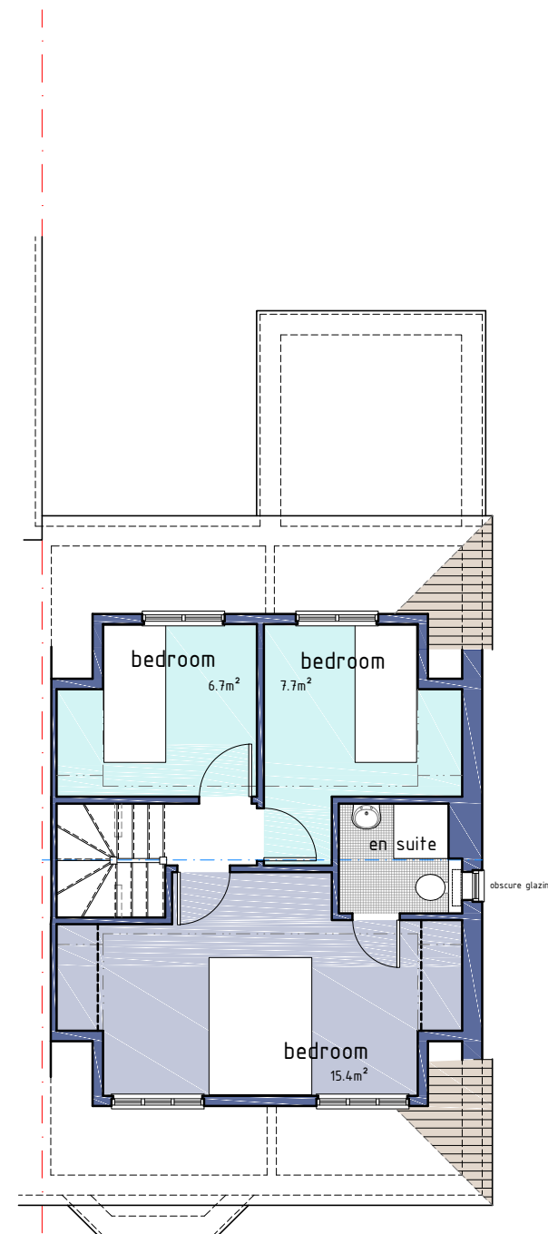
FIRST FLOOR LAYOUT PLAN
