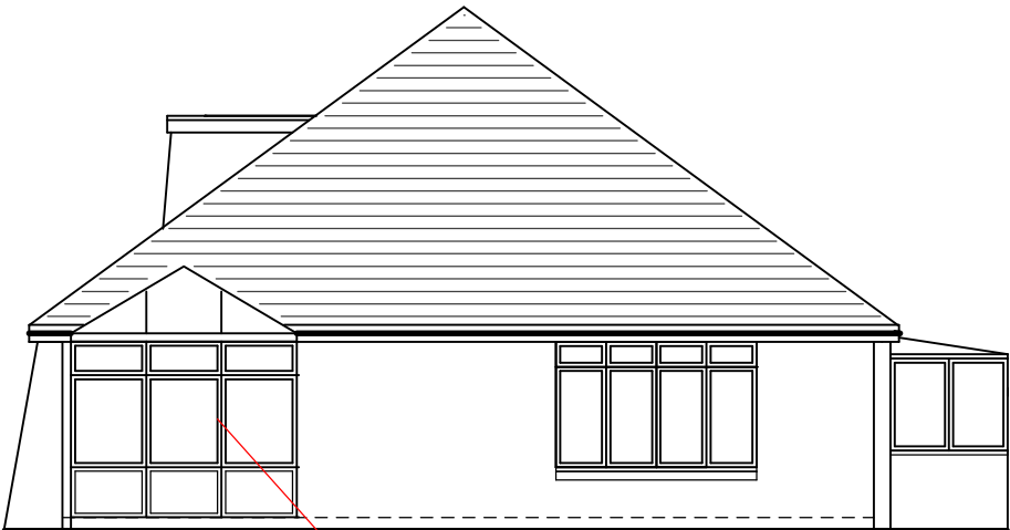
right (south east) elevation
