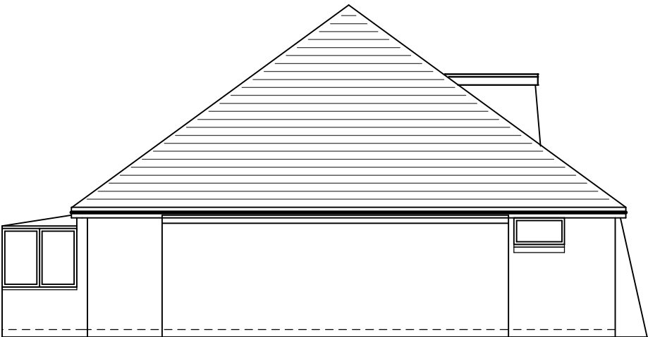
left (north west) elevation
