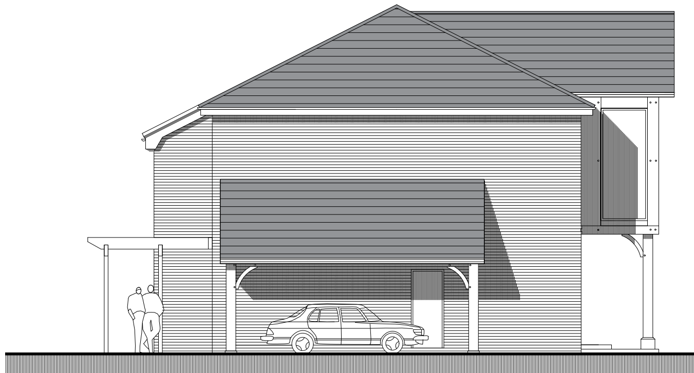
SOUTH ELEVATION
