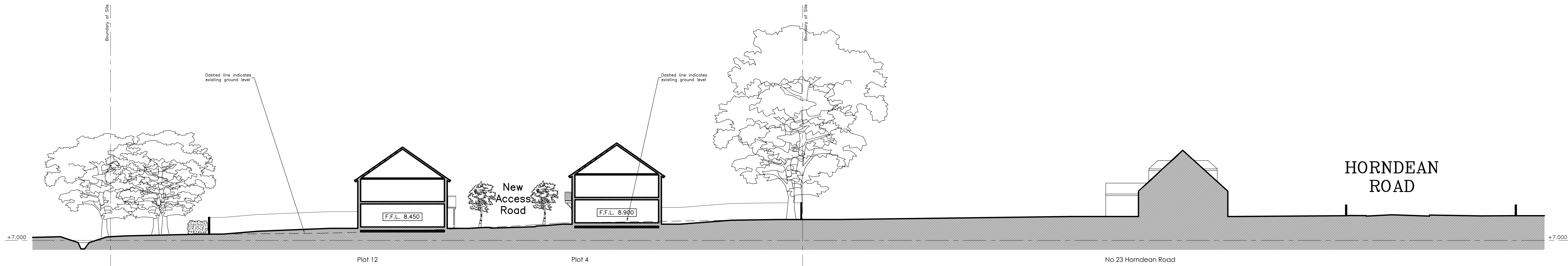
Cross Section Through Central Part of Site (From Plot 12 through to Plot 4)
