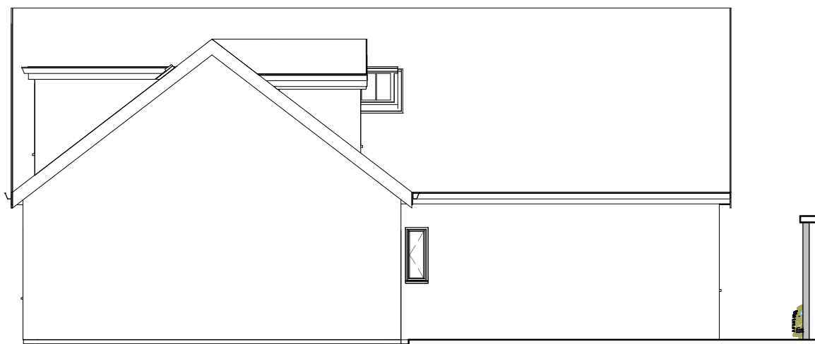
3 South Elevation 1 : 100
