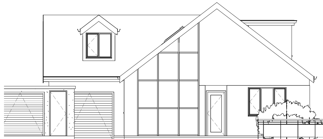
1 East Elevation 1 : 100
