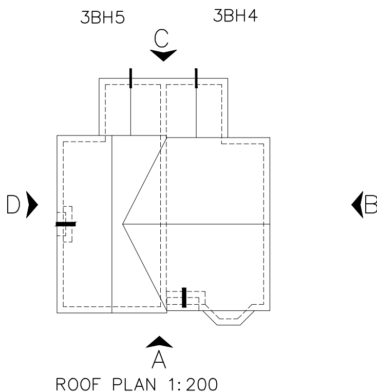
ROOF PLAN 1:200
