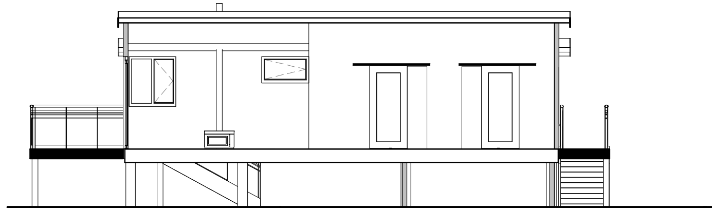
2 North south site section 1 : 100
