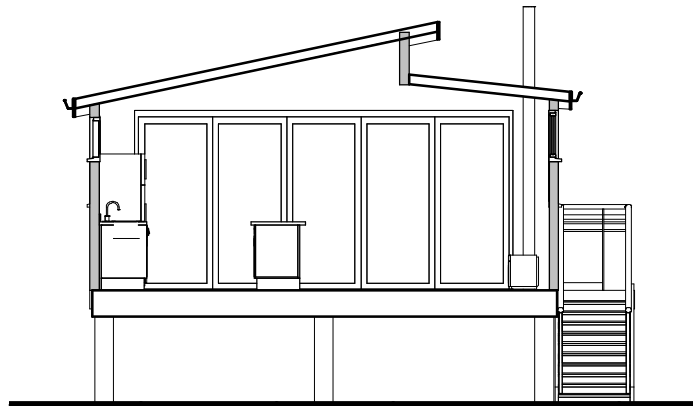
1 East west site section 1 : 100
