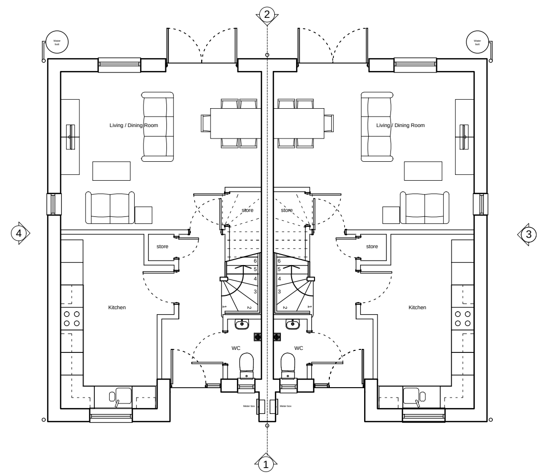
01 Ground Floor Plan 2005 Scale: 1:100
