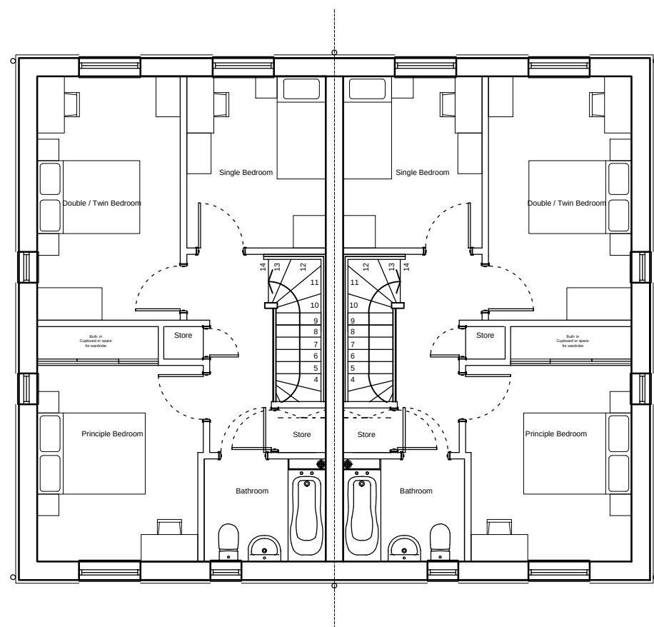
02 First Floor Plan 2005 Scale: 1:100
