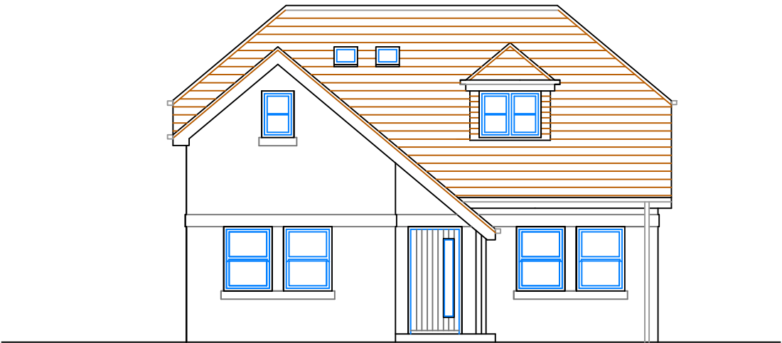
West Elevation
