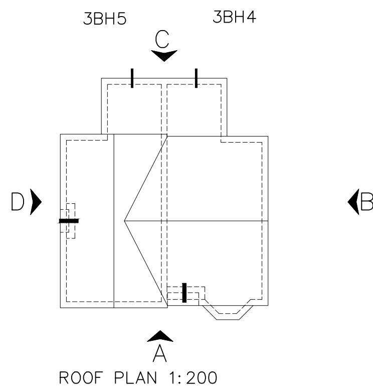
ROOF PLAN 1:200
