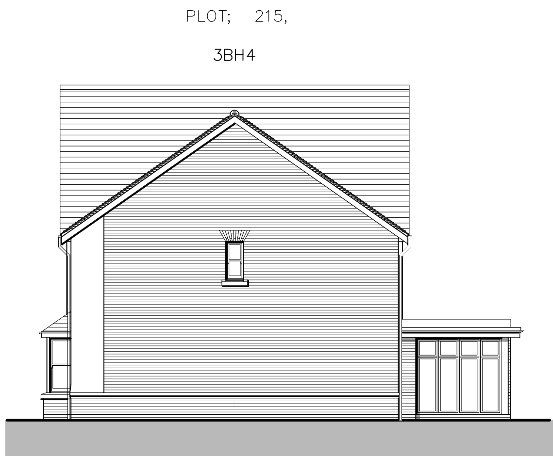
SIDE ELEVATION – B
