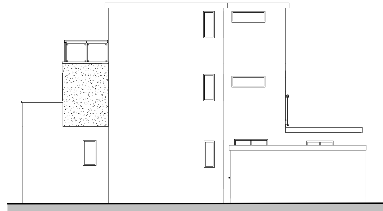
Existing NW Elevation
