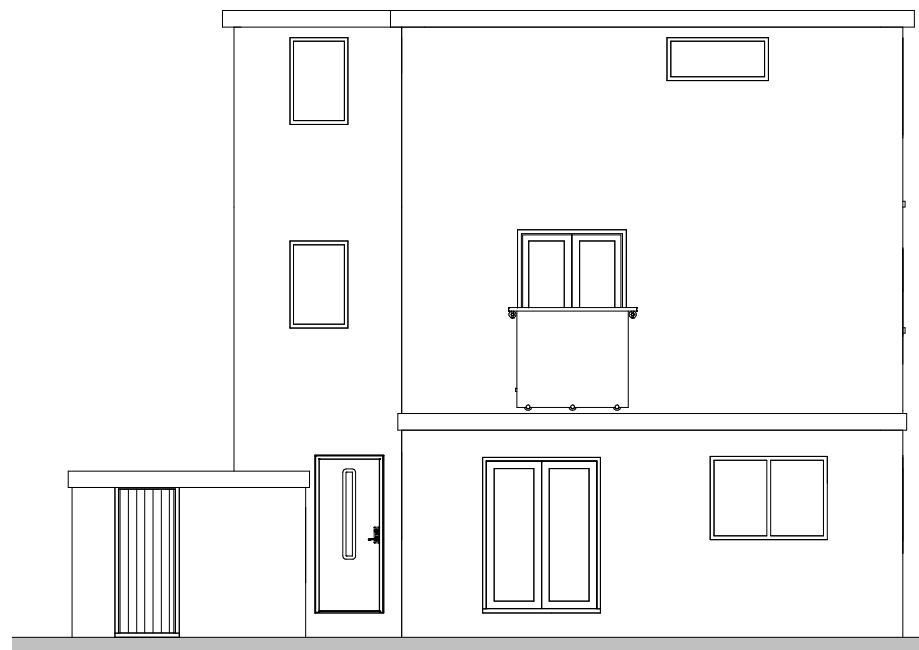
Existing SW Elevation
