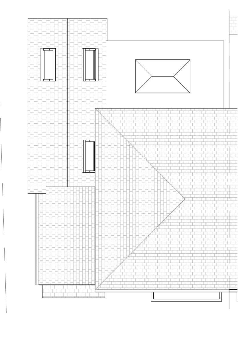
05/304 – PROPOSED ROOF PLAN 1 : 100
