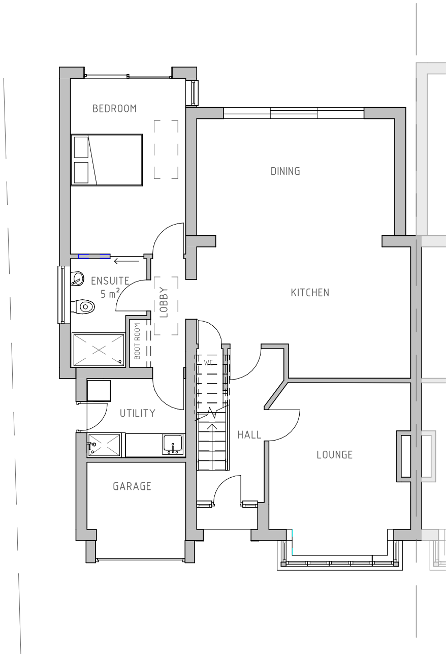
05/301 – PROPOSED GROUND FLOOR PLAN 1 : 100
