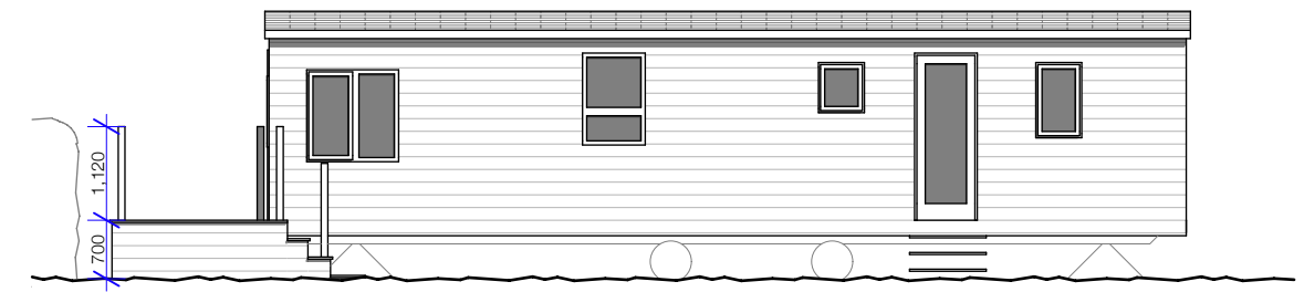
Side (West) elevation 1:100
