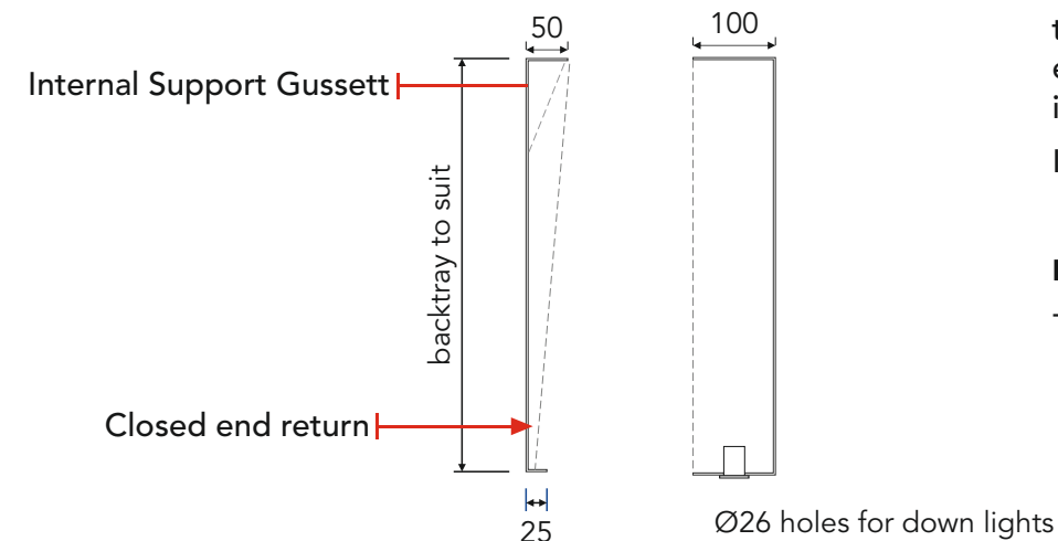
A-A Section Detail Scale 1:10
