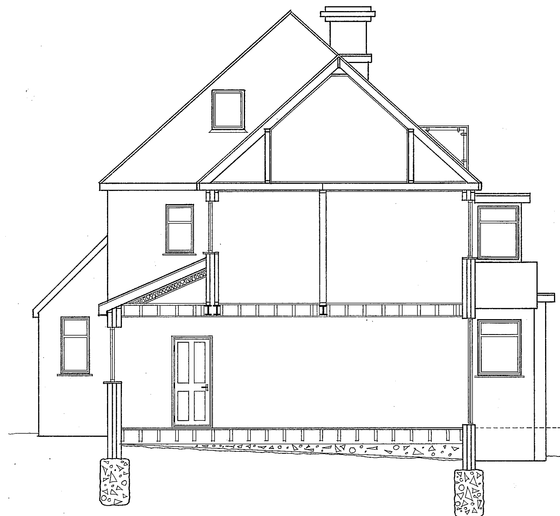
SECTION - BB
