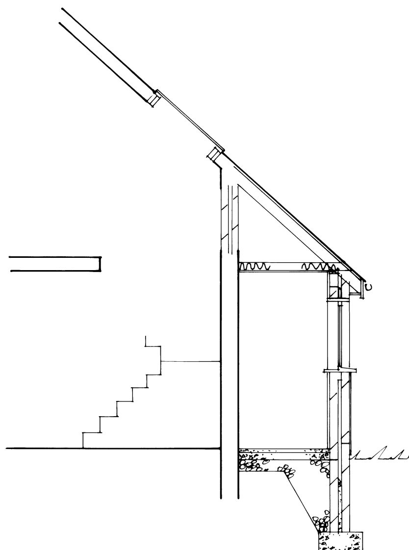
Cross-Section
