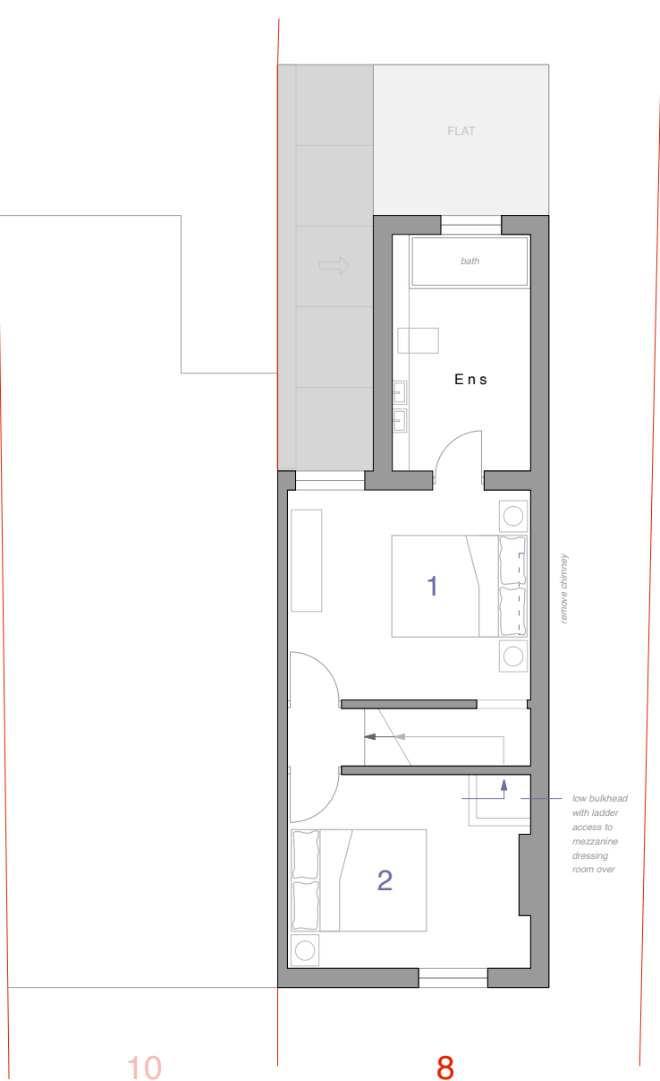
KING'S ROAD Proposed First Floor Plan at 1:100 scale
