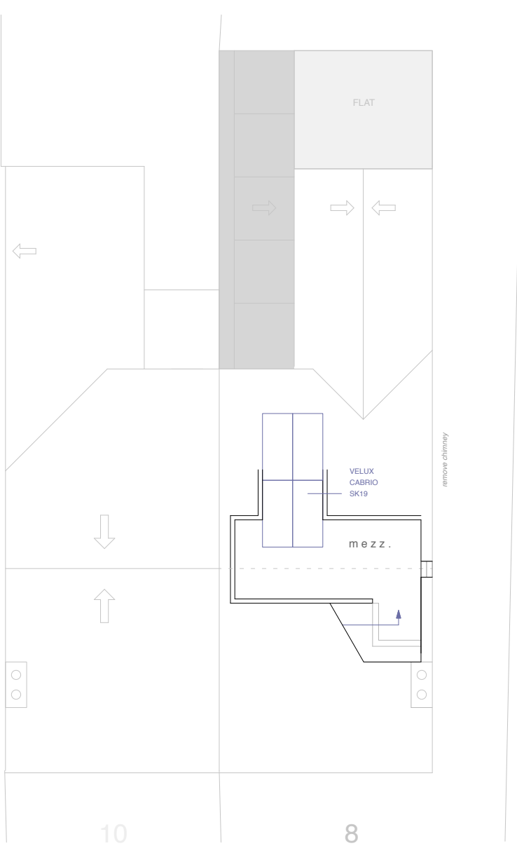
KING'S ROAD Proposed Loft Plan at 1:100 scale
