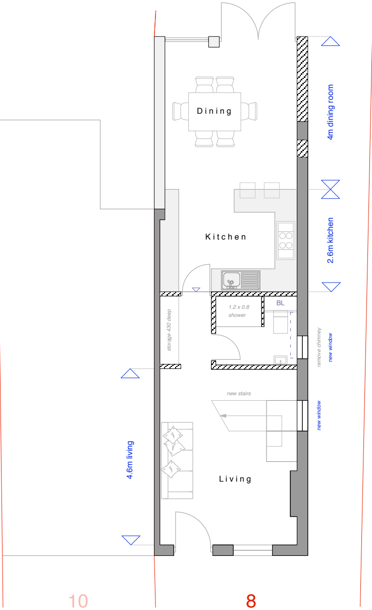
KING'S ROAD Proposed Ground Floor Plan at 1:100 scale
