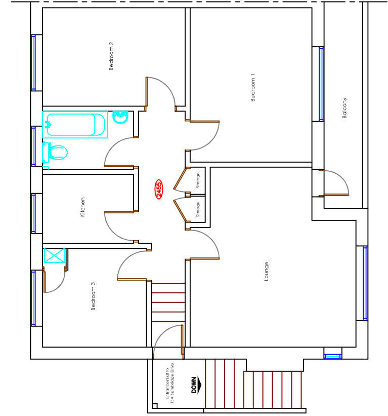
EXISTING FIRST FLOOR (13A Bembridge Drive)
