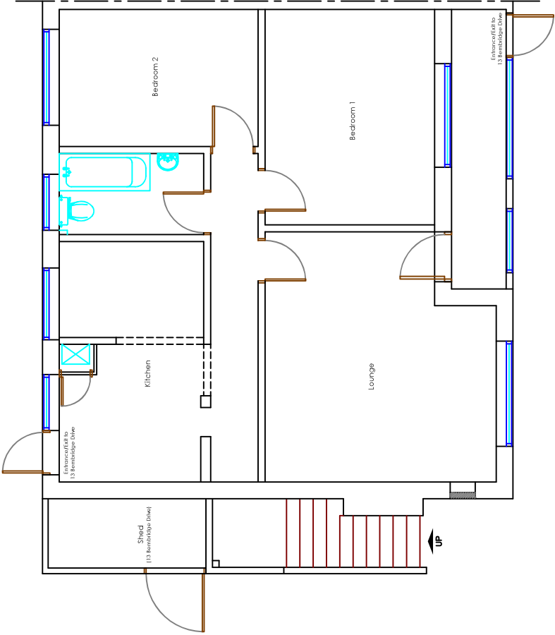
EXISTING GROUND FLOOR (13 Bembridge Drive)
