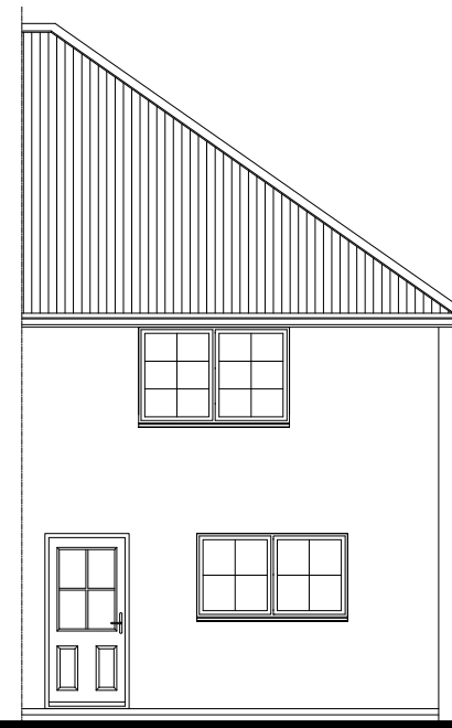
REAR ELEVATION
