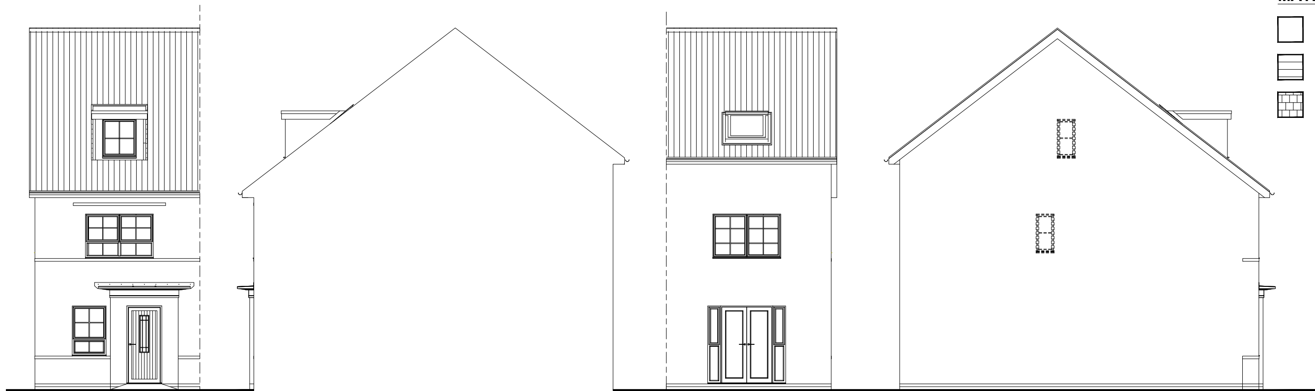
FRONT ELEVATION
