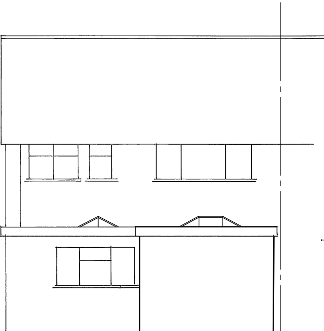
Proposed NE/Rear Elevation
