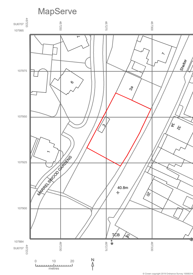
Location Plan
