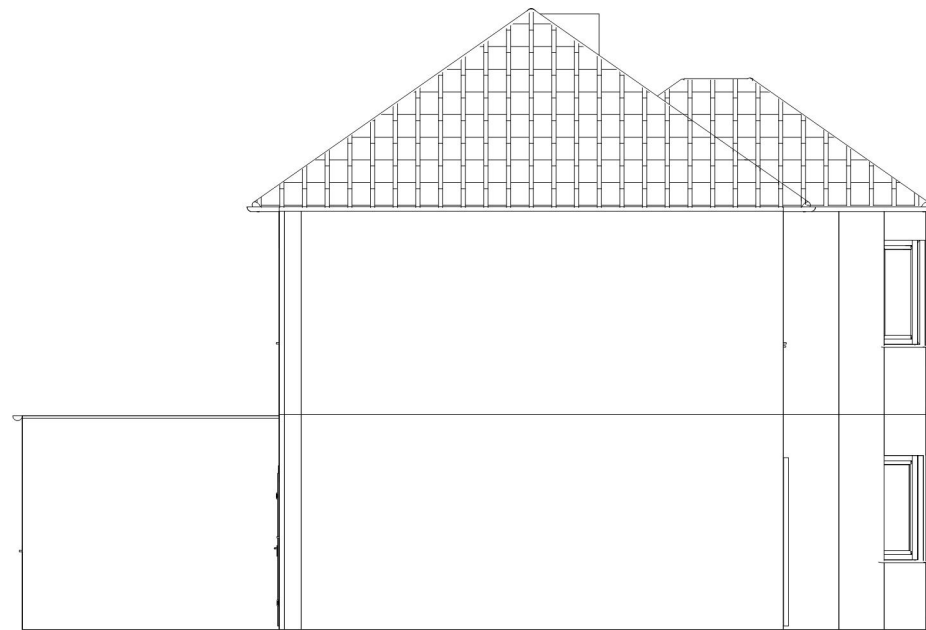
Left Elevation
