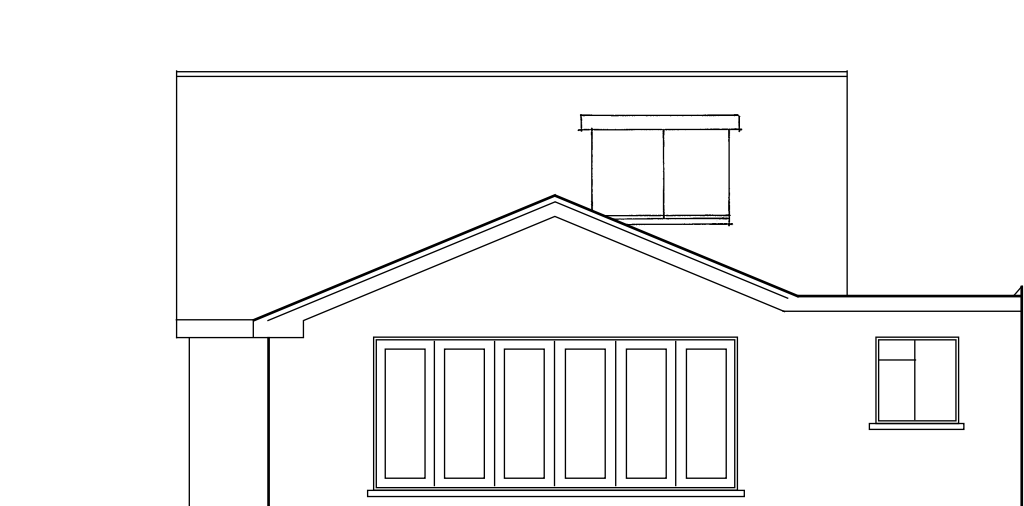
Proposed East/Rear Elevation
