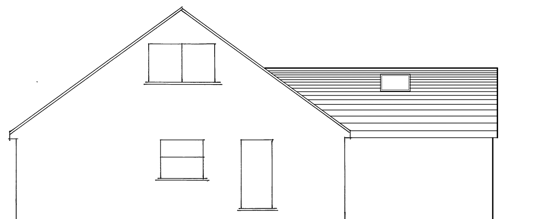
Proposed South/Side Elevation
