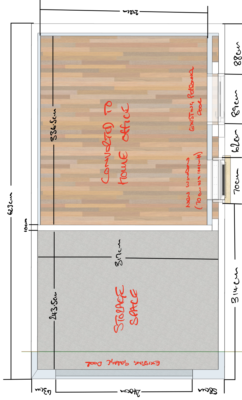
Plan of garage conversion
