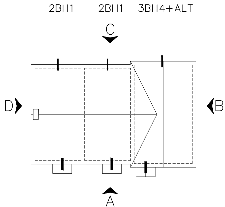
ROOF PLAN 1:200
