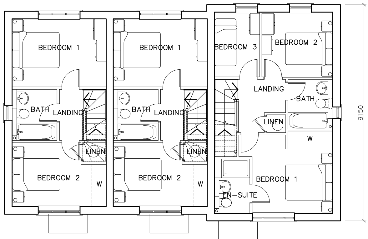
FIRST FLOOR
