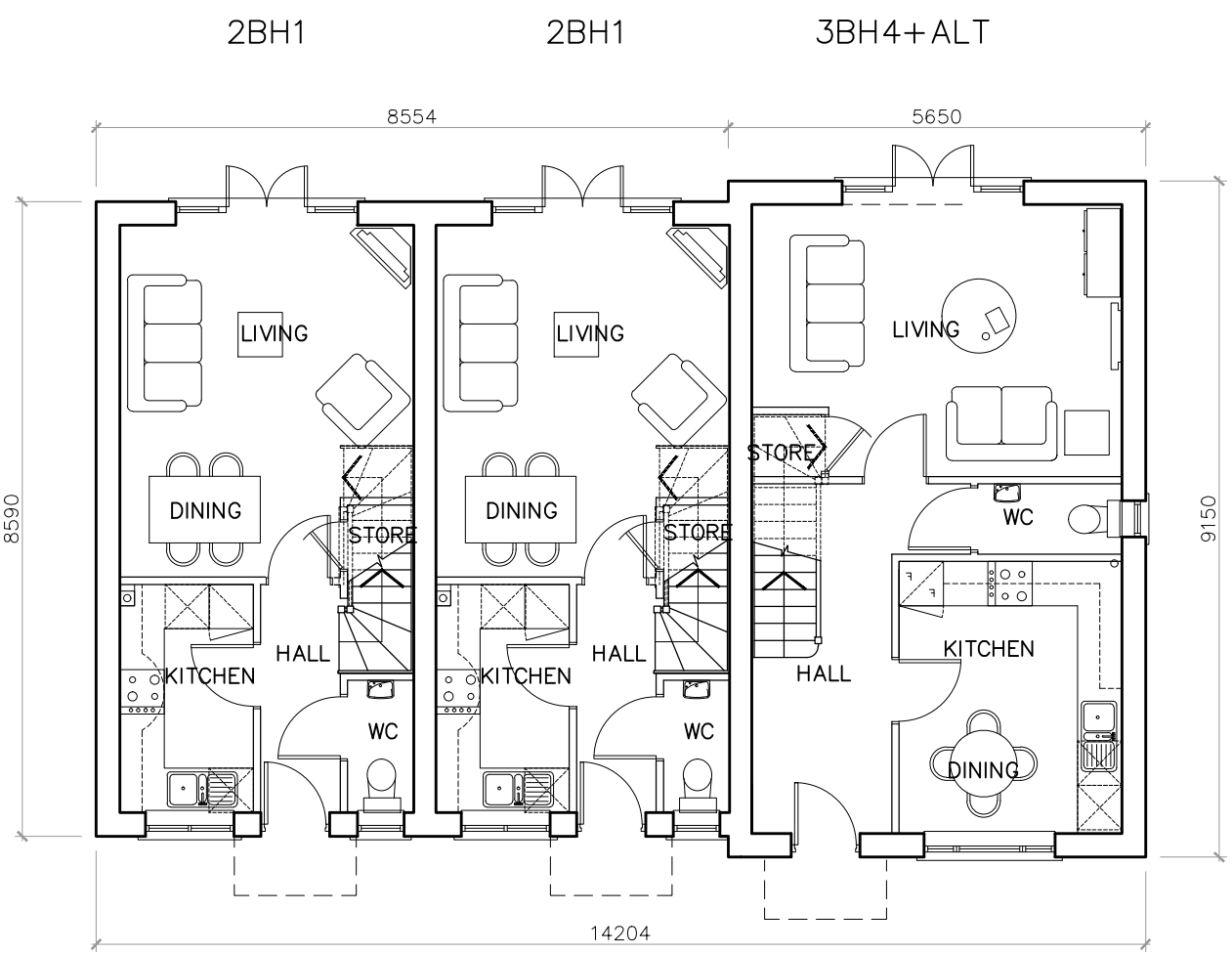
GROUND FLOOR PLOT 135–h, 136,199 PLOT 134–h,137,200 PLOT 133–h,138,201
