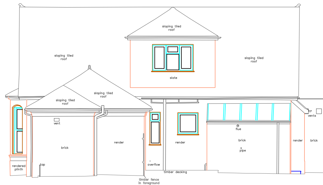
Front Elevation to Durham Gardens
