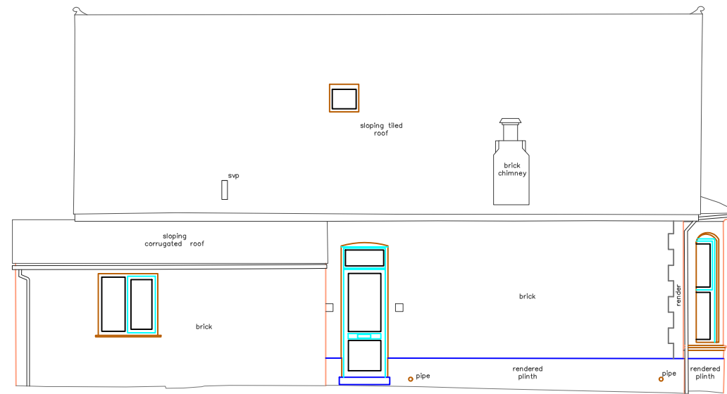
Front Elevation to Durham Gardens
