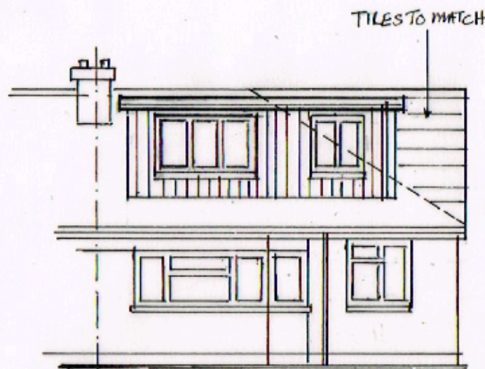
FRONT (SOUTH)
