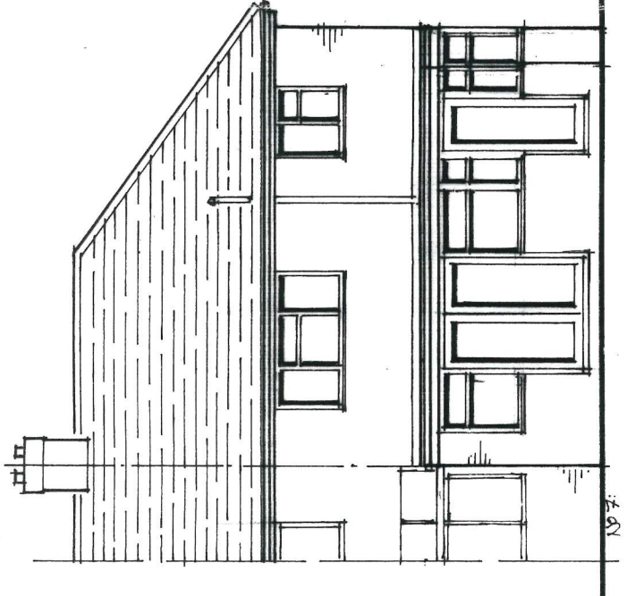
East Elevation
