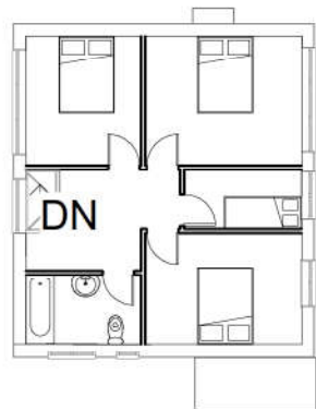
Existing 1st Floor Plan
