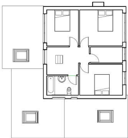
Proposed 1st Floor Plan
