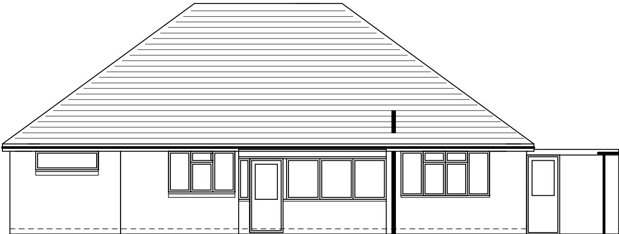
rear (north east) elevation
