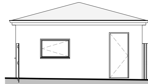
5 Office C South Elevation 1 : 100
