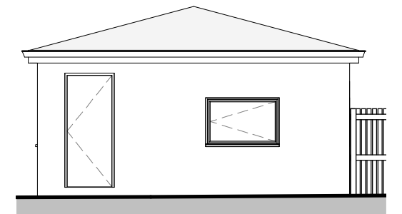
6 Office C West Elevation 1 : 100
