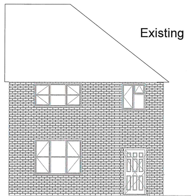
South Elevations
