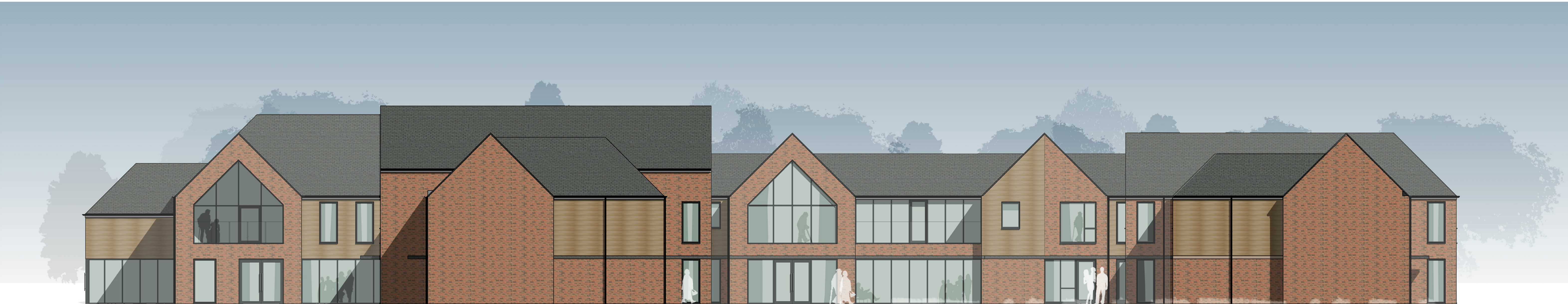
SOUTH ELEVATION 1:100
