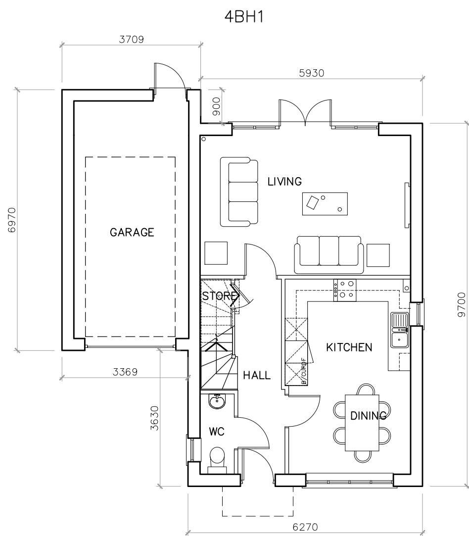
GROUND FLOOR
