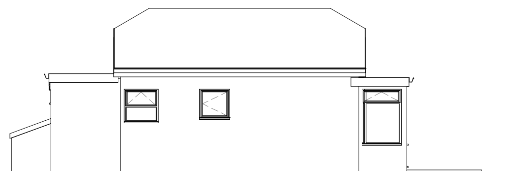
5 South East Elevation
