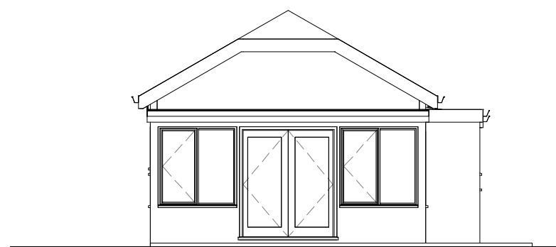
2 North East Elevation
