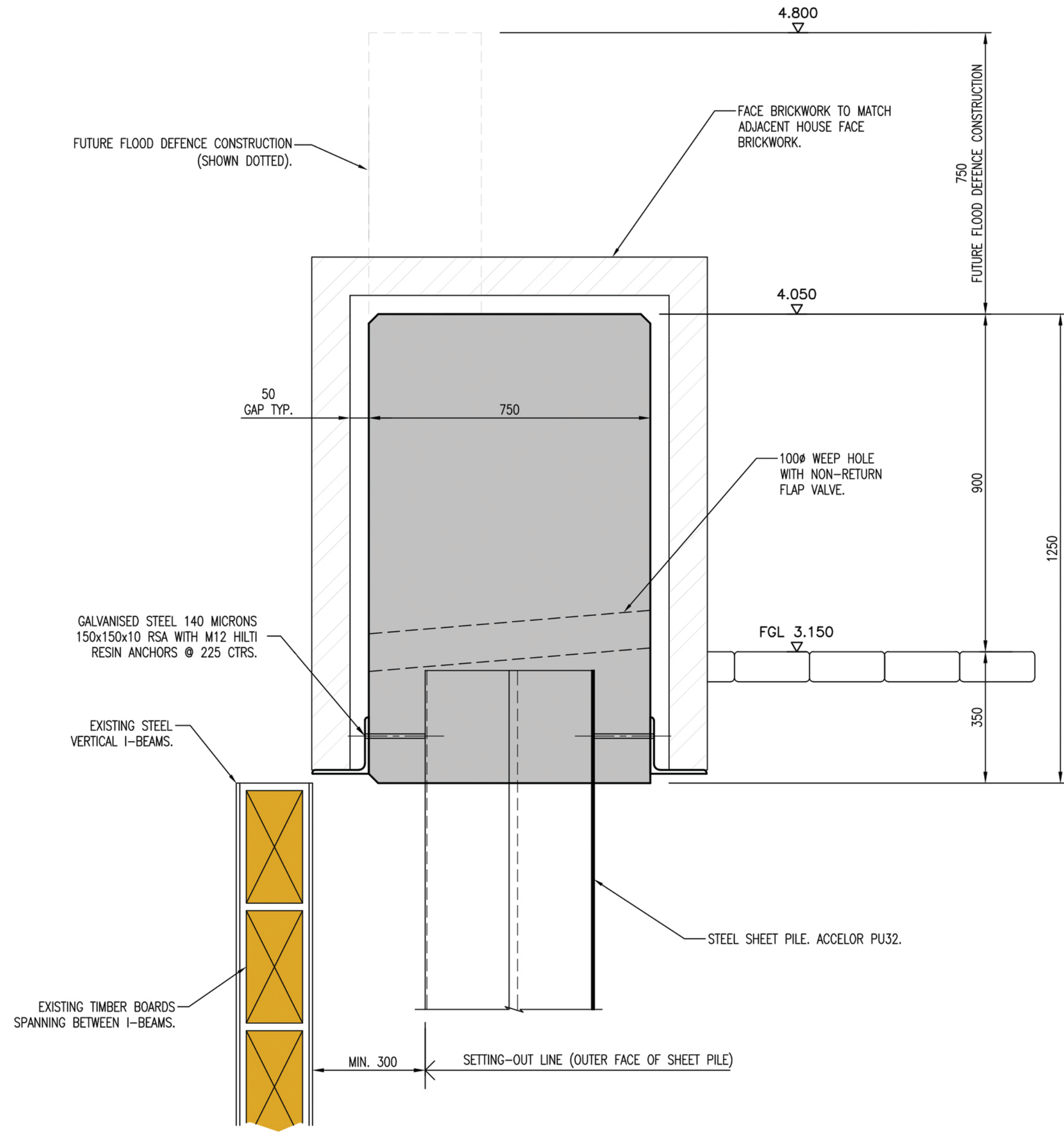
DETAIL C – TYPICAL DEFENCE WALL DETAIL. SCALE 1:10
