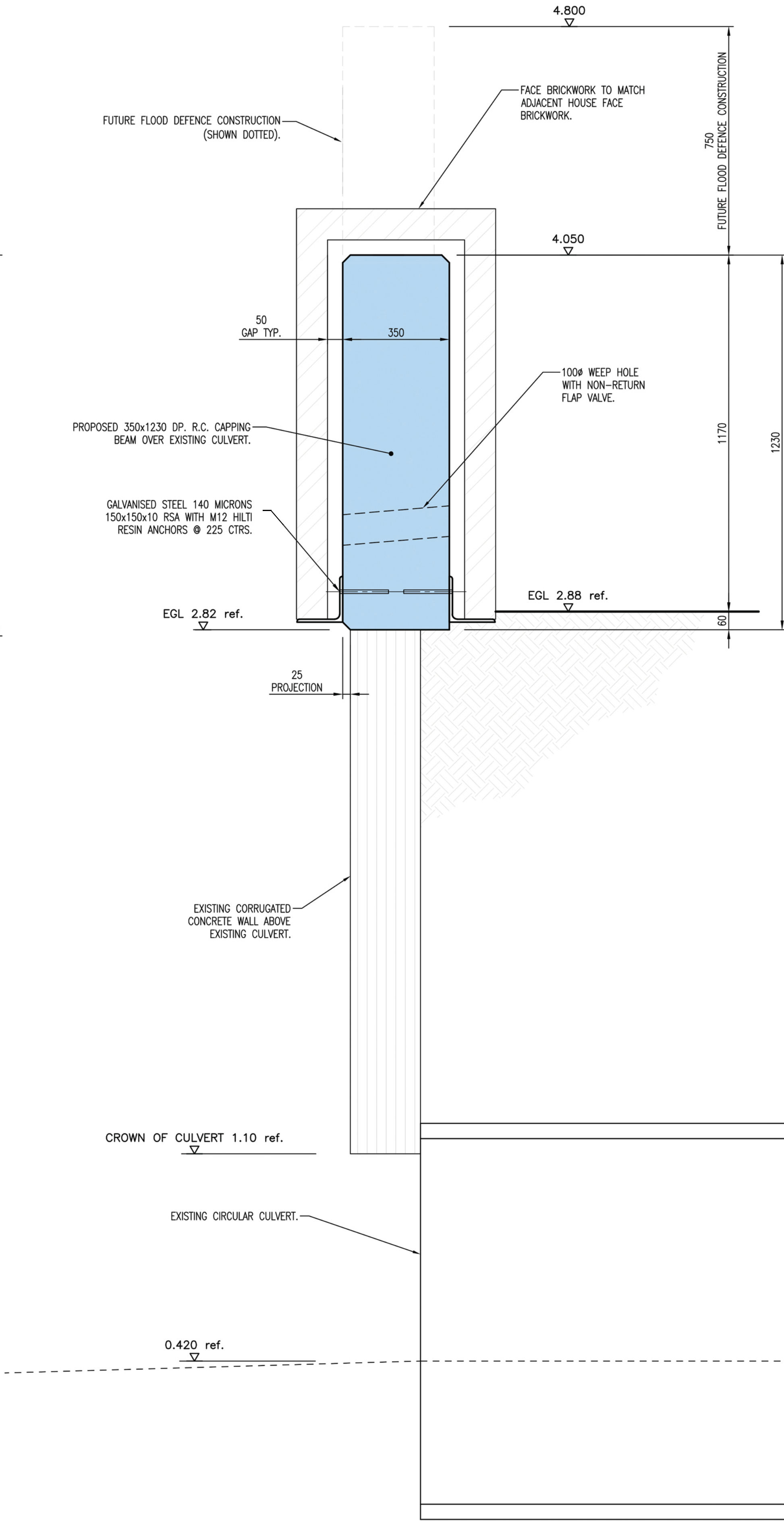
DETAIL D SECTION THROUGH EXISTING CULVERT. SCALE 1:10
