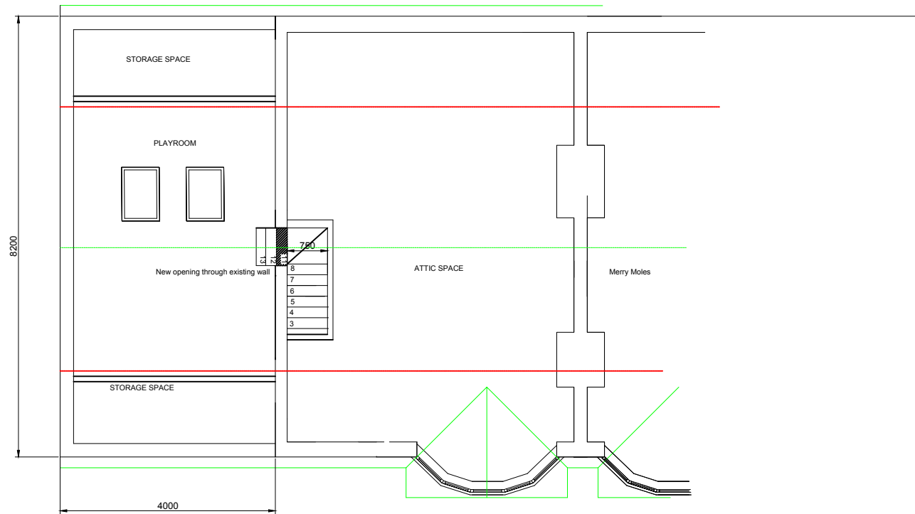
PROPOSED ATTIC FLOOR PLAN 1:100
