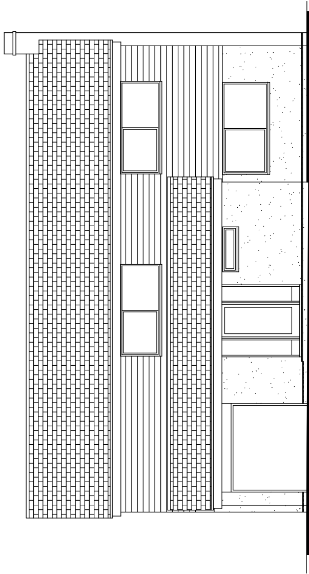
FRONT (NORTH)
