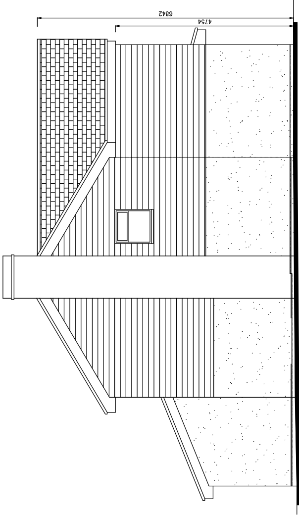
RIGHT (WEST)
