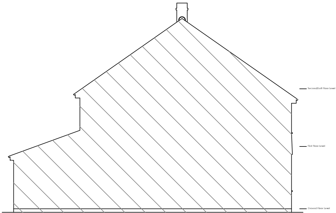
EXISTING SIDE SECTION/ELEVATION
