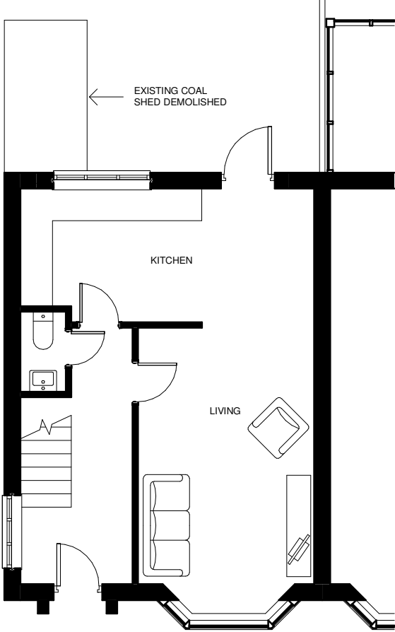
P-003 EXISTING GROUND FLOOR PLAN 1 : 100
