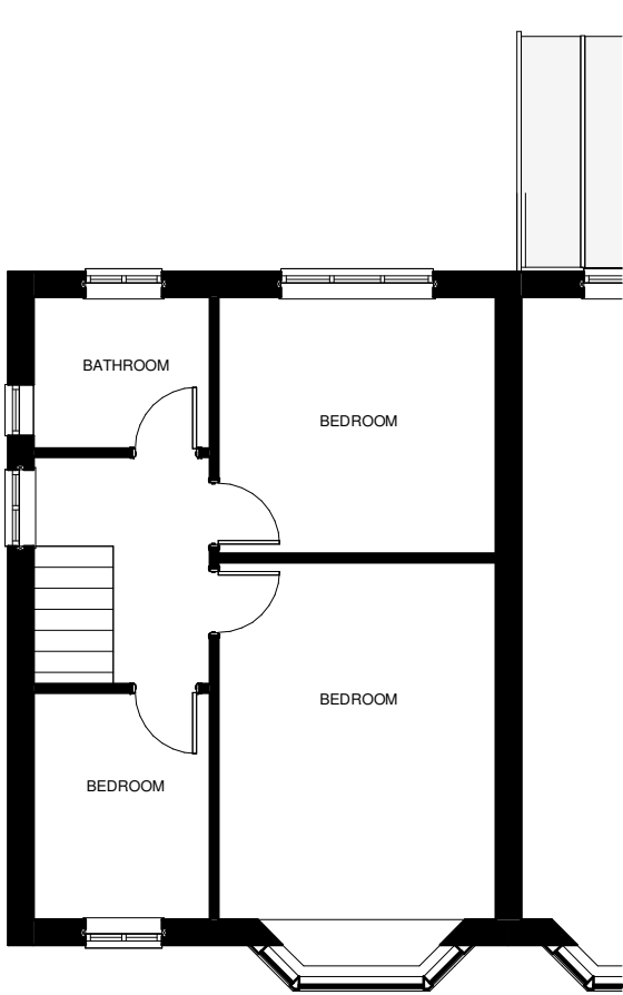
P-003 EXISTING FIRST FLOOR PLAN 1 : 100
